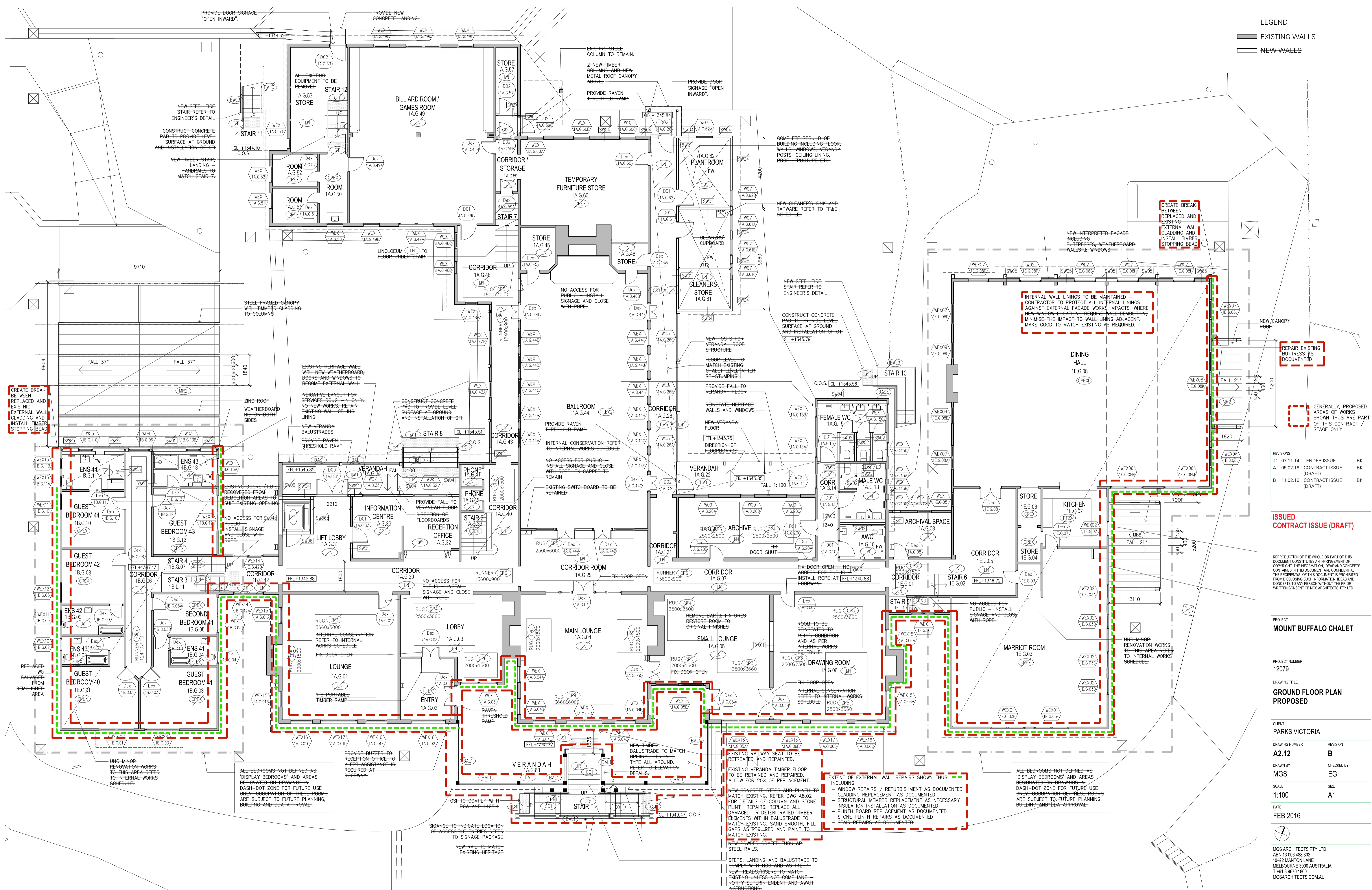
01 GROUND FLOOR PLAN - PROPOSED 1:100 @ A1 - 1:200 @ A3
